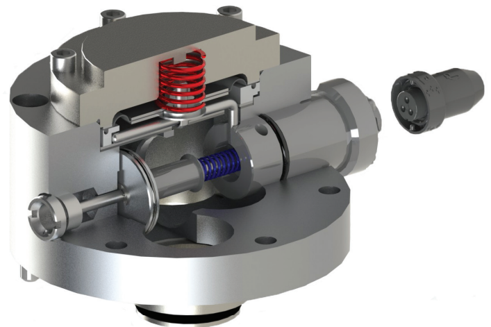
Bypass open
