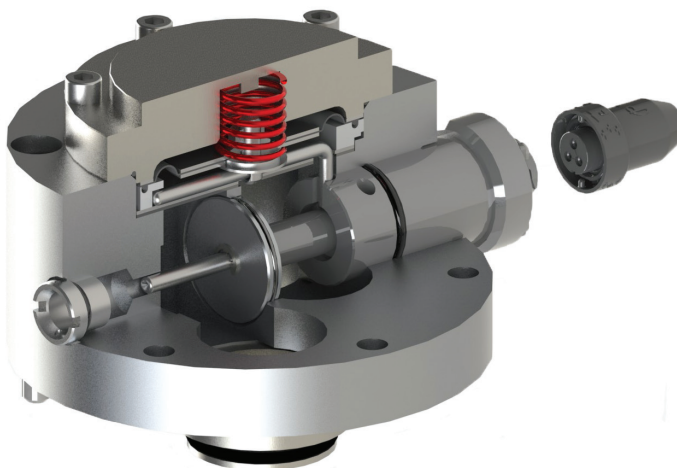
Bypass closed
